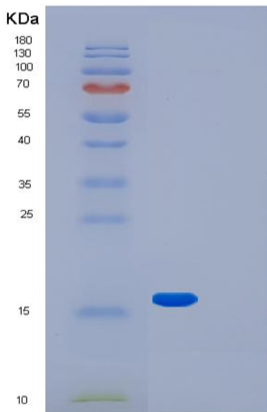
Figure 2. SDS-PAGE
