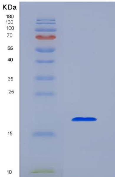
Figure 2. SDS-PAGE
