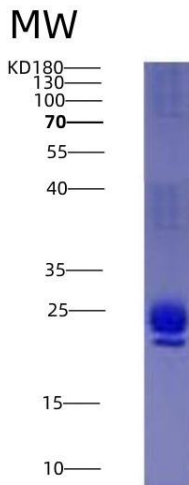
Figure 2. SDS-PAGE
