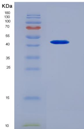
Figure 2. SDS-PAGE
