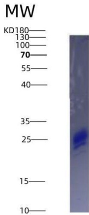
Figure 1. SDS-PAGE
