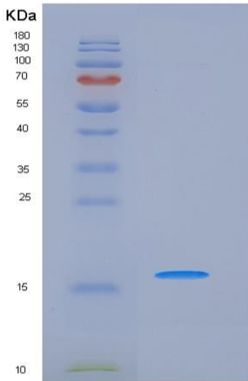
Figure 1. SDS-PAGE
