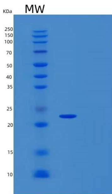
Figure . SDS-PAGE
