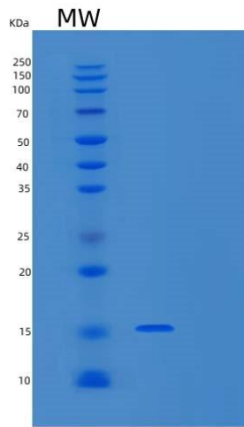
Figure 2. SDS-PAGE
