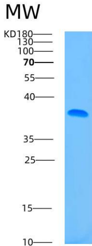
Figure 1. SDS-PAGE
