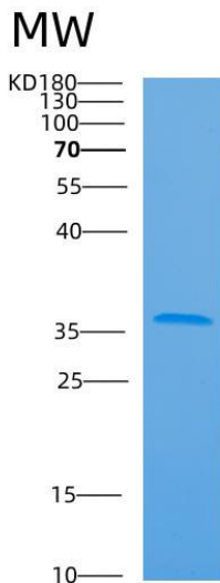
Figure 1. SDS-PAGE
