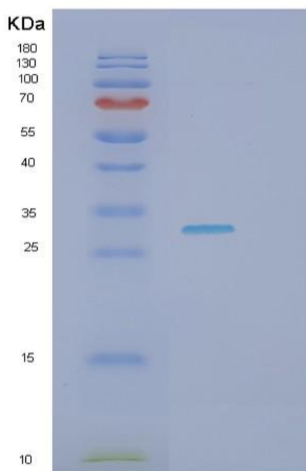
Figure . SDS-PAGE
