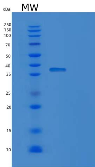
Figure 1. SDS-PAGE
