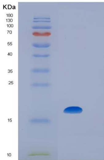
Figure 1. SDS-PAGE
