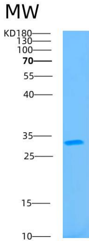
Figure 1. SDS-PAGE
