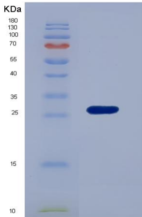
Figure 1. SDS-PAGE
