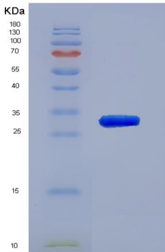
Figure 2. SDS-PAGE
