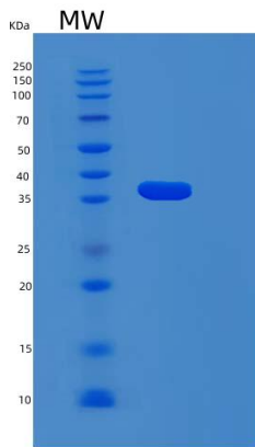
Figure 1. SDS-PAGE
