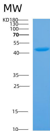
Figure 2. SDS-PAGE
