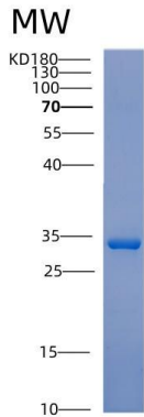
Figure 1. SDS-PAGE
