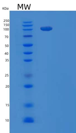
Figure 1. SDS-PAGE
