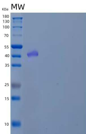
Figure 1. SDS-PAGE
