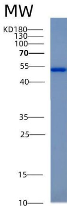
Figure 1. SDS-PAGE
