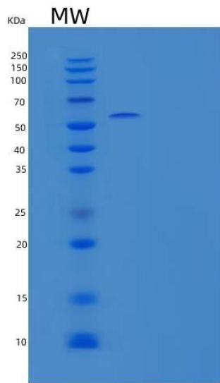
Figure 1. SDS-PAGE
