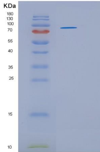
Figure 1. SDS-PAGE
