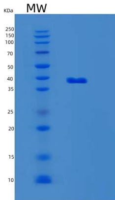
Figure 1. SDS-PAGE
