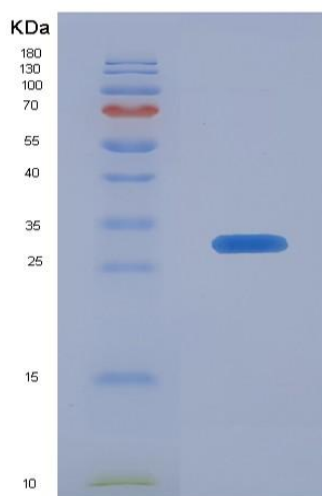
Figure . SDS-PAGE
