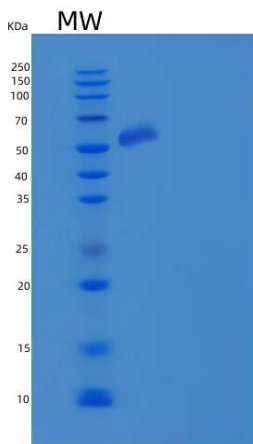
Figure 1. SDS-PAGE
