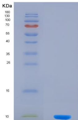
Figure . SDS-PAGE
