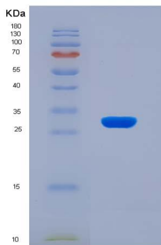
Figure . SDS-PAGE
