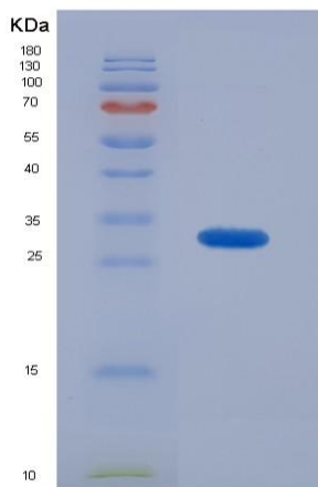
Figure . SDS-PAGE
