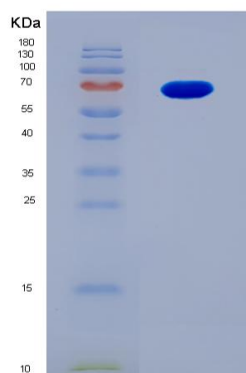
Figure . SDS-PAGE
