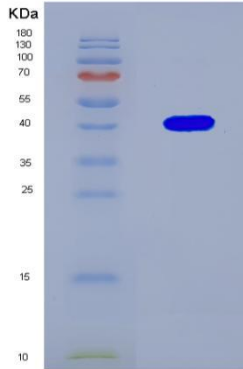
Figure . SDS-PAGE
