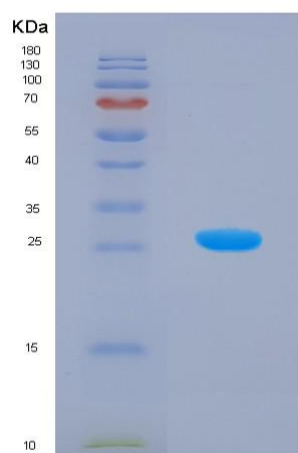
Figure 1. SDS-PAGE
