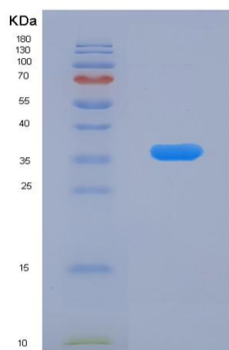
Figure . SDS-PAGE
