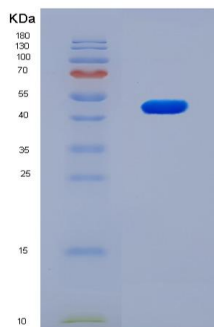
Figure 1. SDS-PAGE
