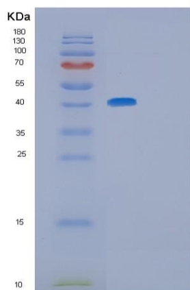
Figure . SDS-PAGE
