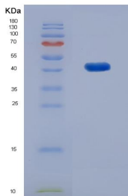
Figure 1. SDS-PAGE
