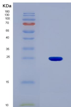
Figure 1. SDS-PAGE
