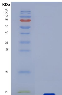
Figure 1. SDS-PAGE
