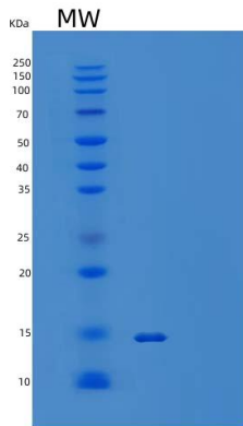
Figure 1. SDS-PAGE
